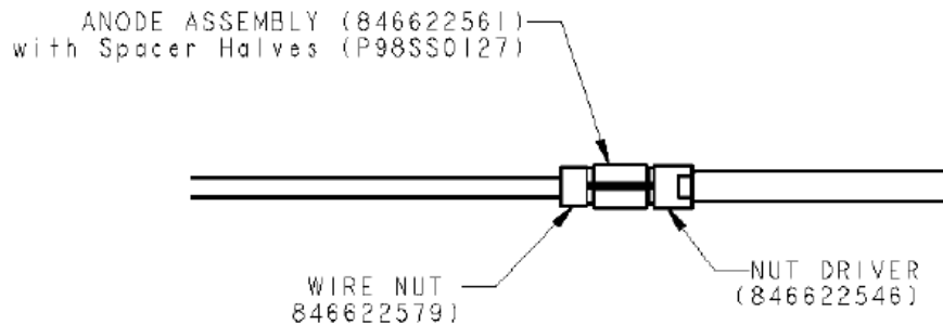
Figure 1 – Anode Screen Termination (with Spacer Halves)
