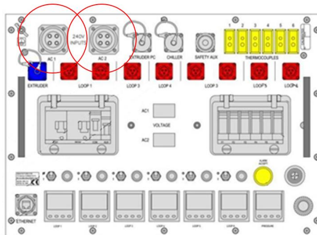
Figure 1 – 240v input sockets identified in red.
